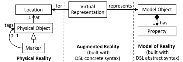
Fig. 2: Augmenting the reality using an AR-based DSL.
