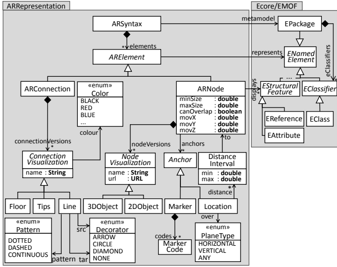
Fig. 3: Meta-model for AR-based concrete syntaxes.
