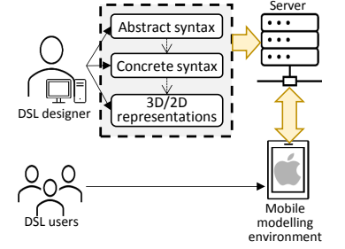
Fig. 4: Architecture of ALTER.
