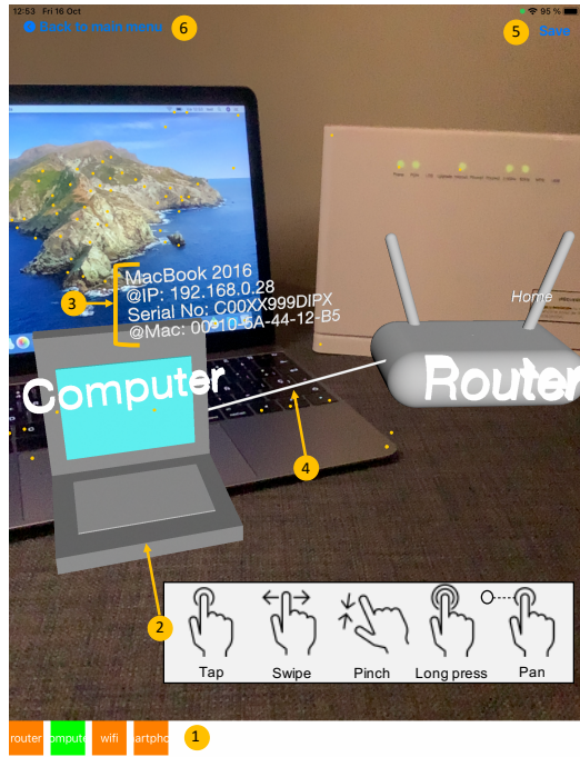
Fig. 5: The main canvas of ALTER (running on an iPad).
